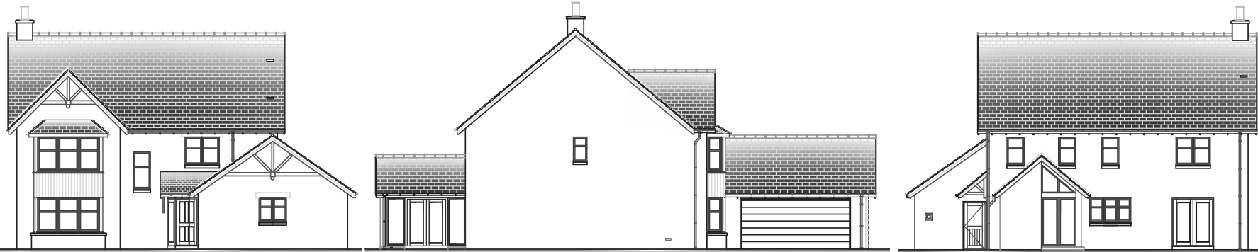
Front Elevation
